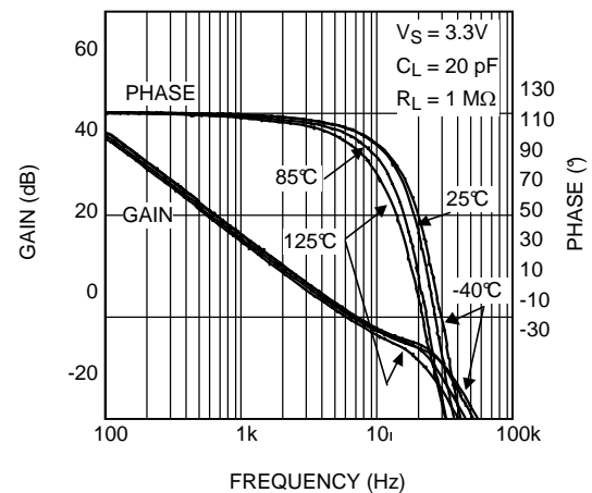
Figure 42. Frequency Response vs. Temperature
