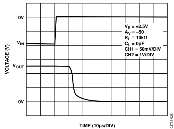
Figure 28. Negative Overtolerance Recovery
