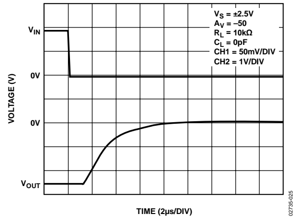
Figure 27. Positive Overtolerance Recovery
