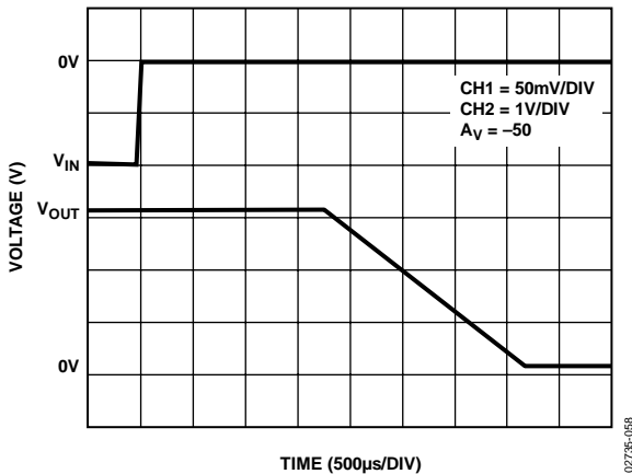
Figure 61. Negative Input Overload Recovery for Competitor B
