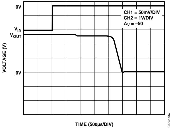
Figure 60. Negative Input Overload Recovery for Competitor A
