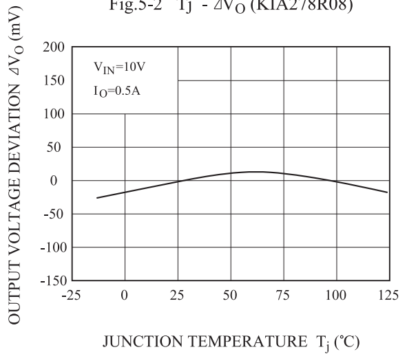
Fig.5-2 T j - ΔV O (KIA278R08)
