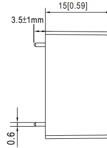
PIN diameter: 0.6 \pm 0.1[0.024 \pm 0.004]
