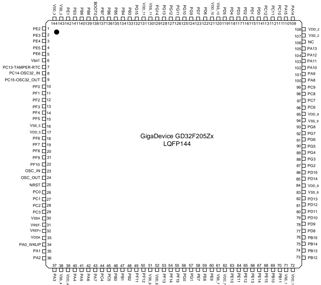
Figure 2. GD32F205Zx LQFP144 pinouts
