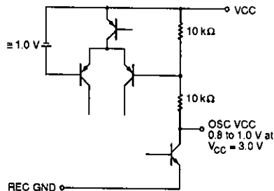
Figure 2. Oscillator supply
