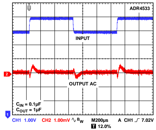
Figure 60. ADR4533 Line Transient Response
