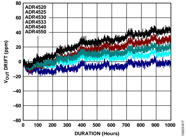
Figure 93. ADR4550 Typical Long-Term Output Voltage Drift (1000 Hours)
