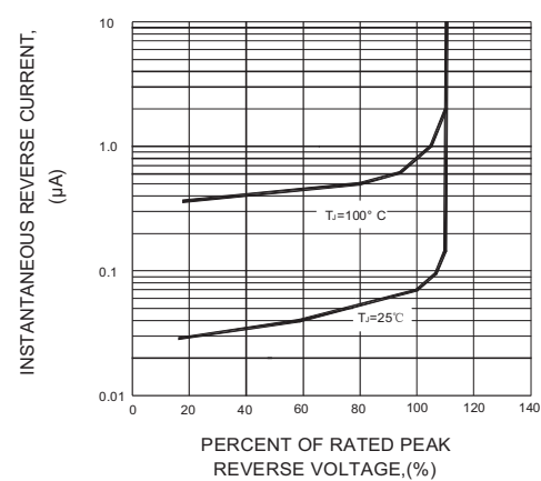
FIG.4-TYPICAL REVERSE CHARACTERISTICS
