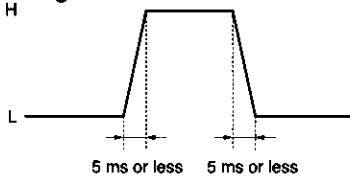
Fig.17 Control signal
