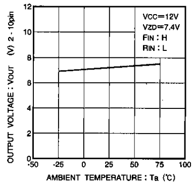
Fig.6 Output voltage vs. ambient temperature (I)
