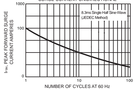
FIG. 6 - MAXIMUM NON-REPETITIVE FORWARD SURGE CURRENT UNIDIRECTIONAL
